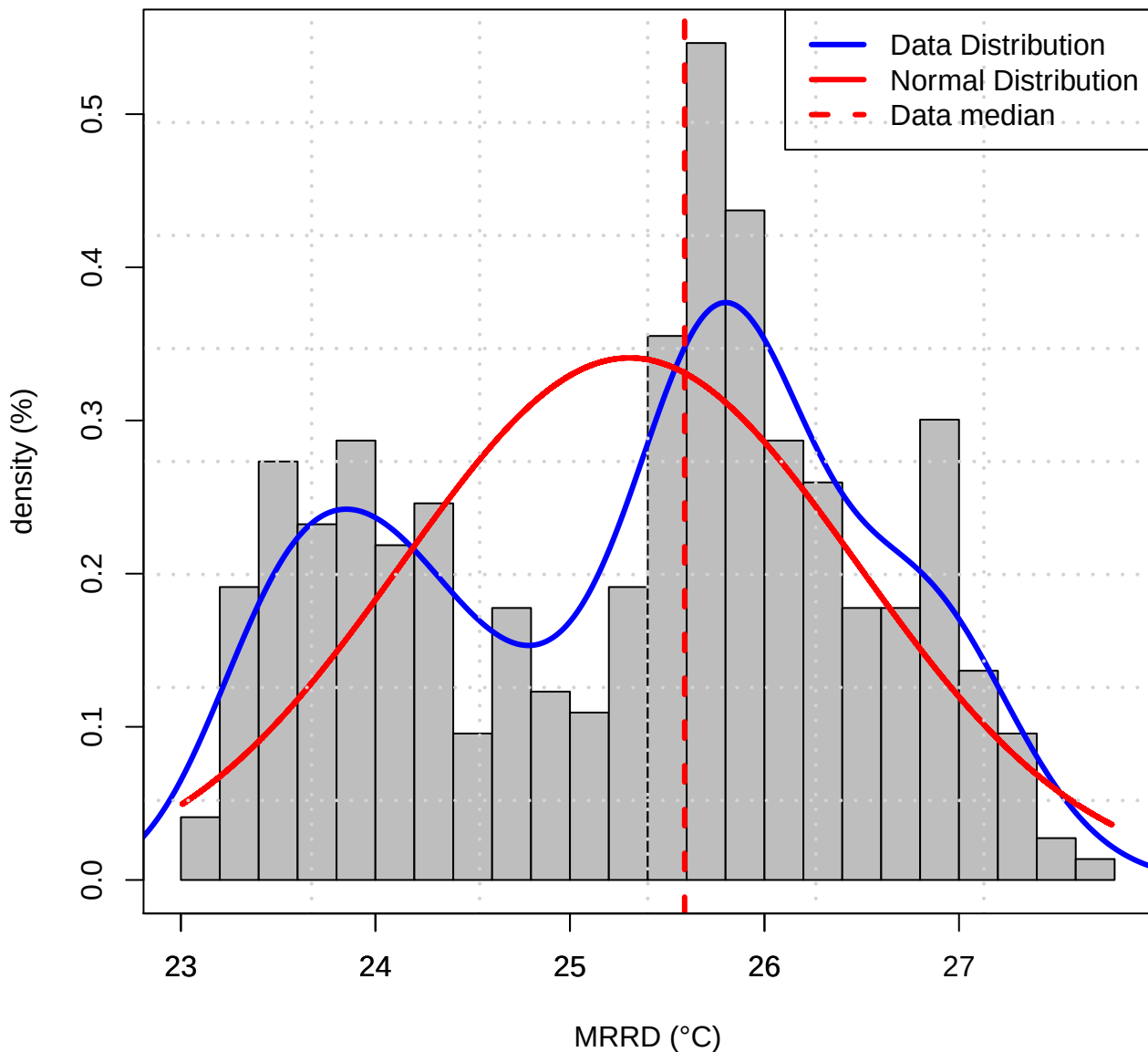
Histogram of Data distribution (TASMAX of MRRD)
