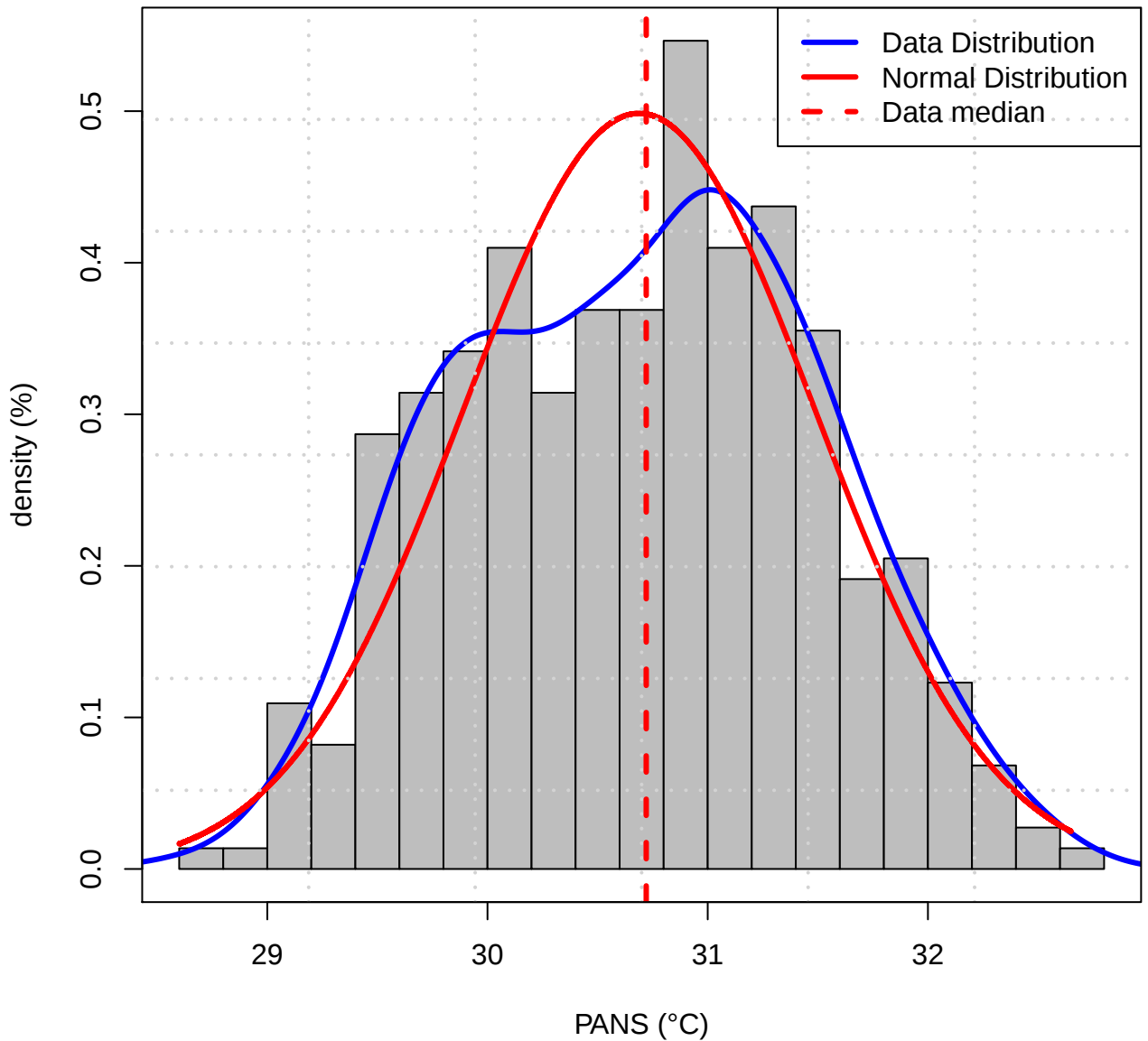
Histogram of Data distribution (TASMAX of PANS)
