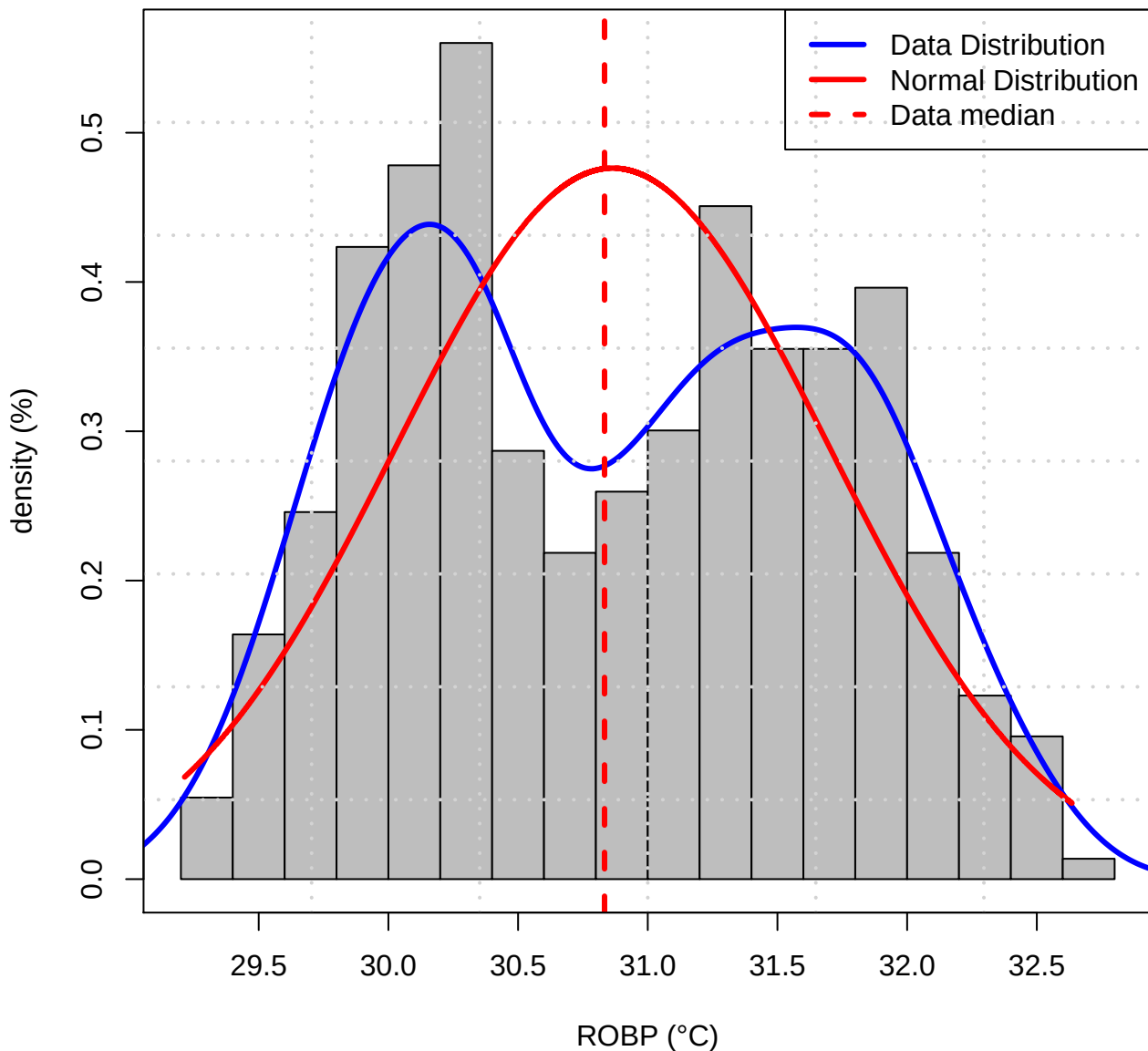
Histogram of Data distribution (TASMAX of ROBP)
