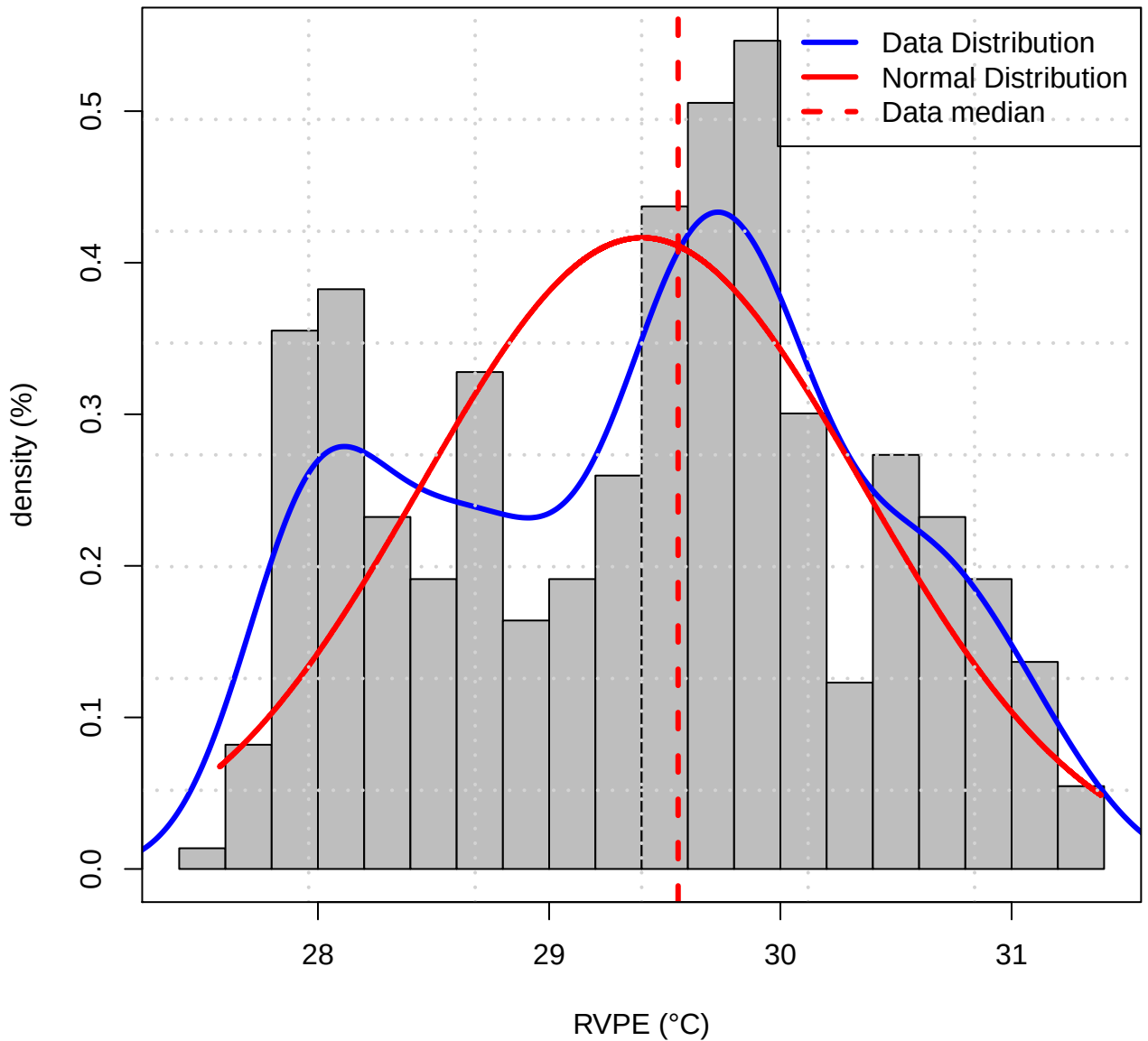
Histogram of Data distribution (TASMAX of RVPE)
