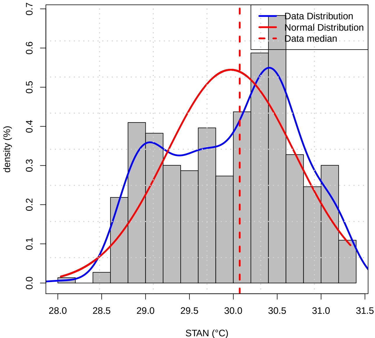
Histogram of Data distribution (TASMAX of STAN)
