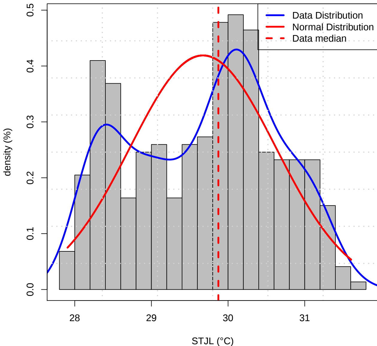
Histogram of Data distribution (TASMAX of STJL)
