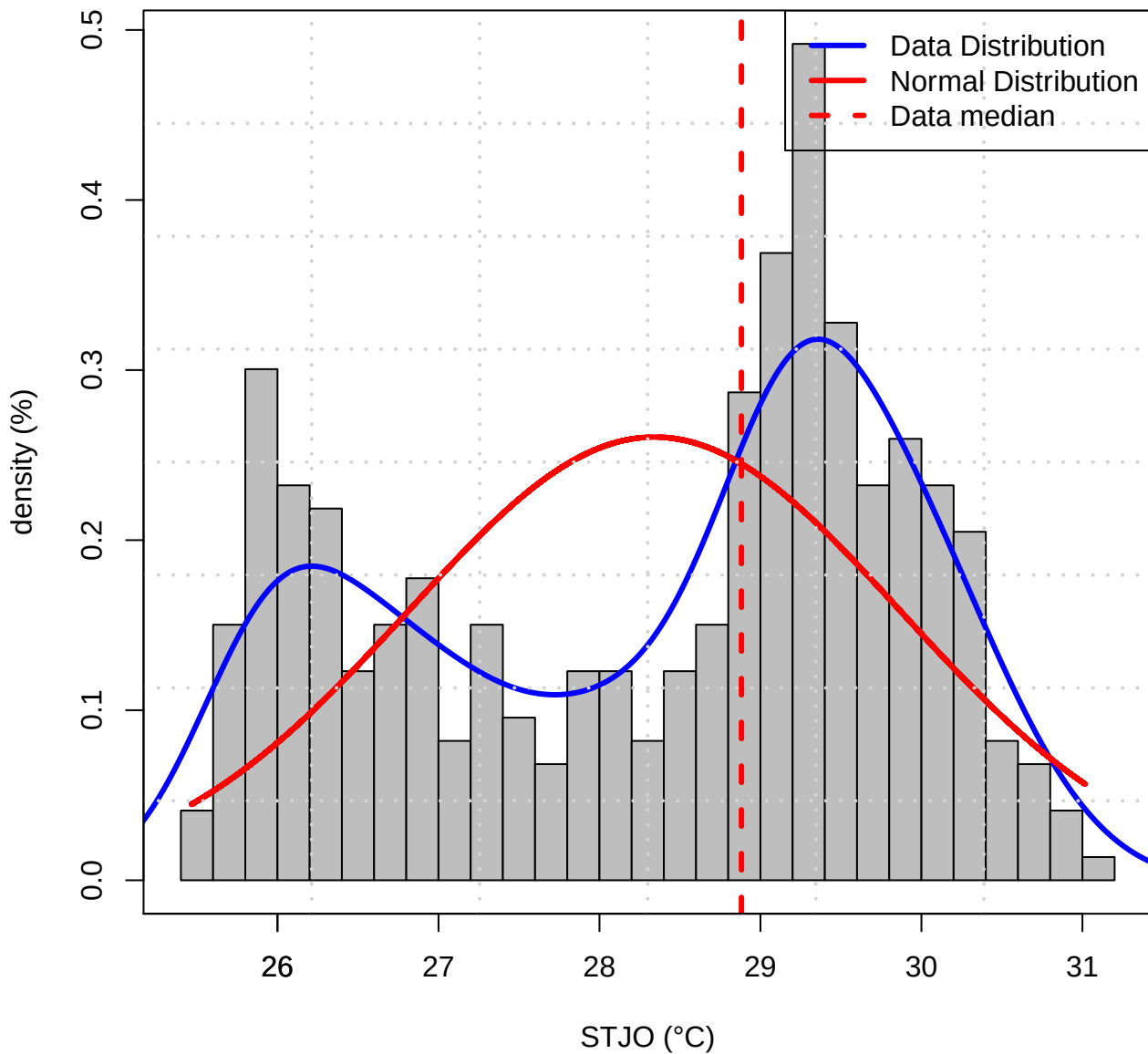
Histogram of Data distribution (TASMAX of STJO)
