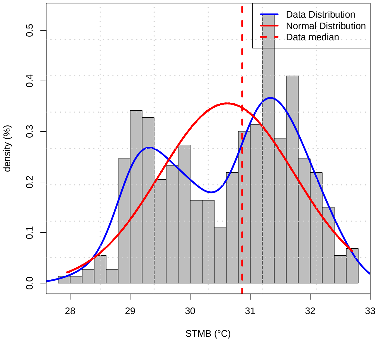
Histogram of Data distribution (TASMAX of STMB)
