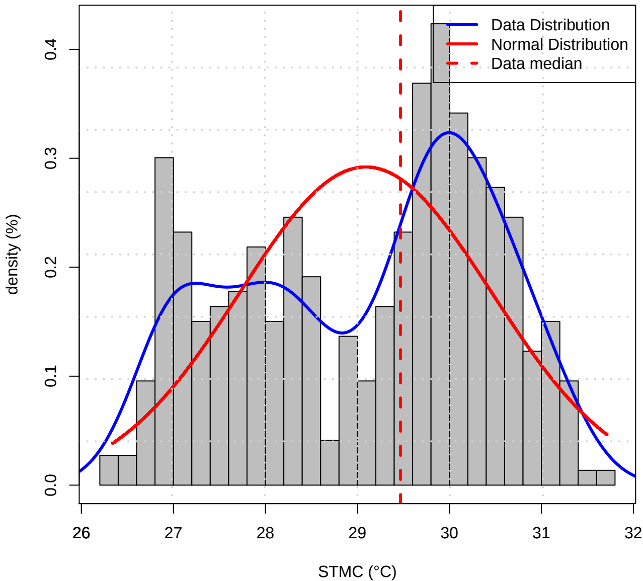
Histogram of Data distribution (TASMAX of STMC)
