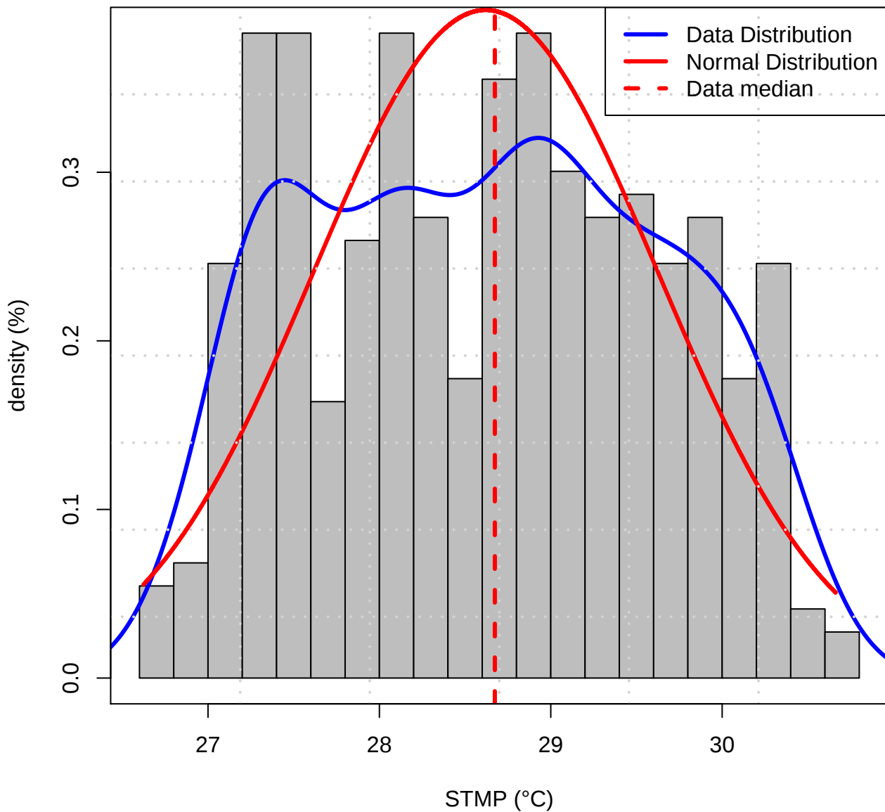
Histogram of Data distribution (TASMAX of STMP)
