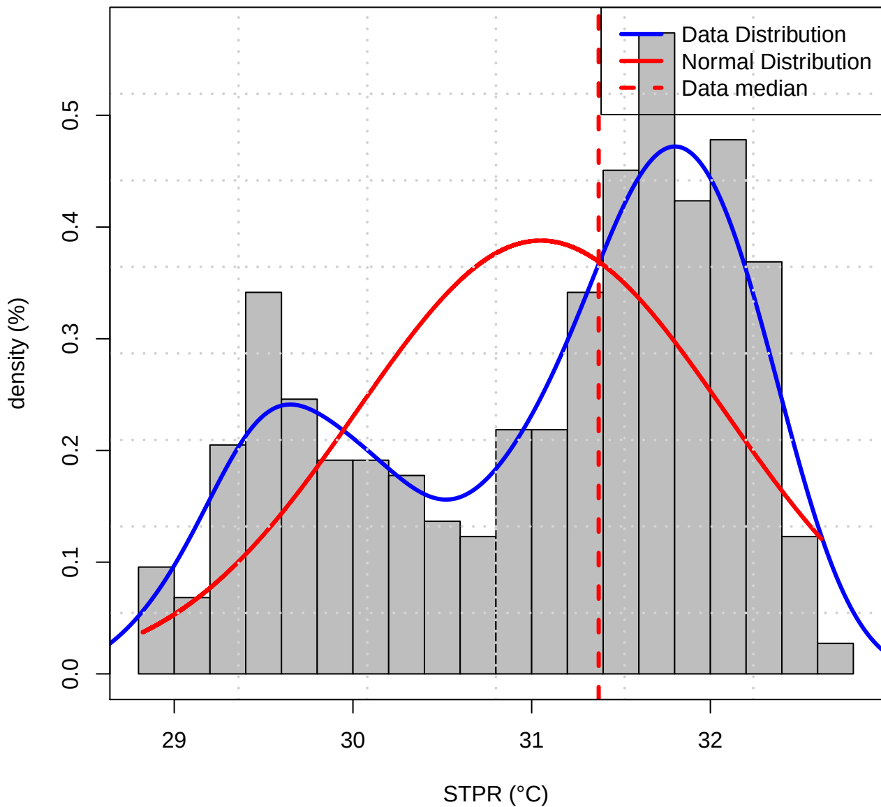
Histogram of Data distribution (TASMAX of STPR)
