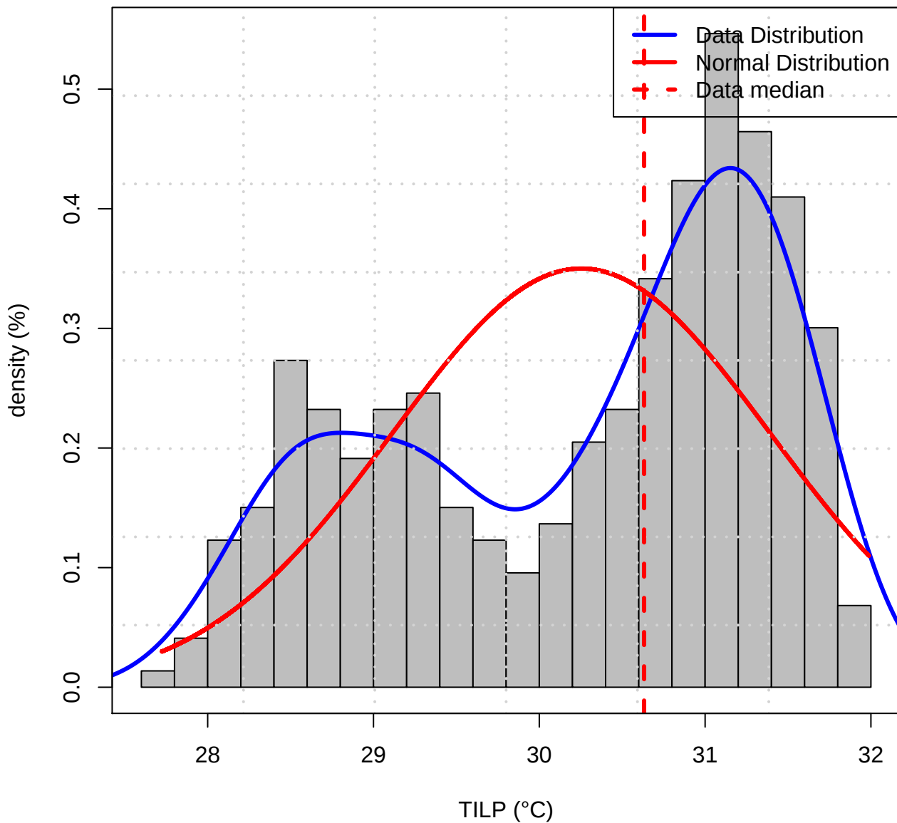
Histogram of Data distribution (TASMAX of TILP)
