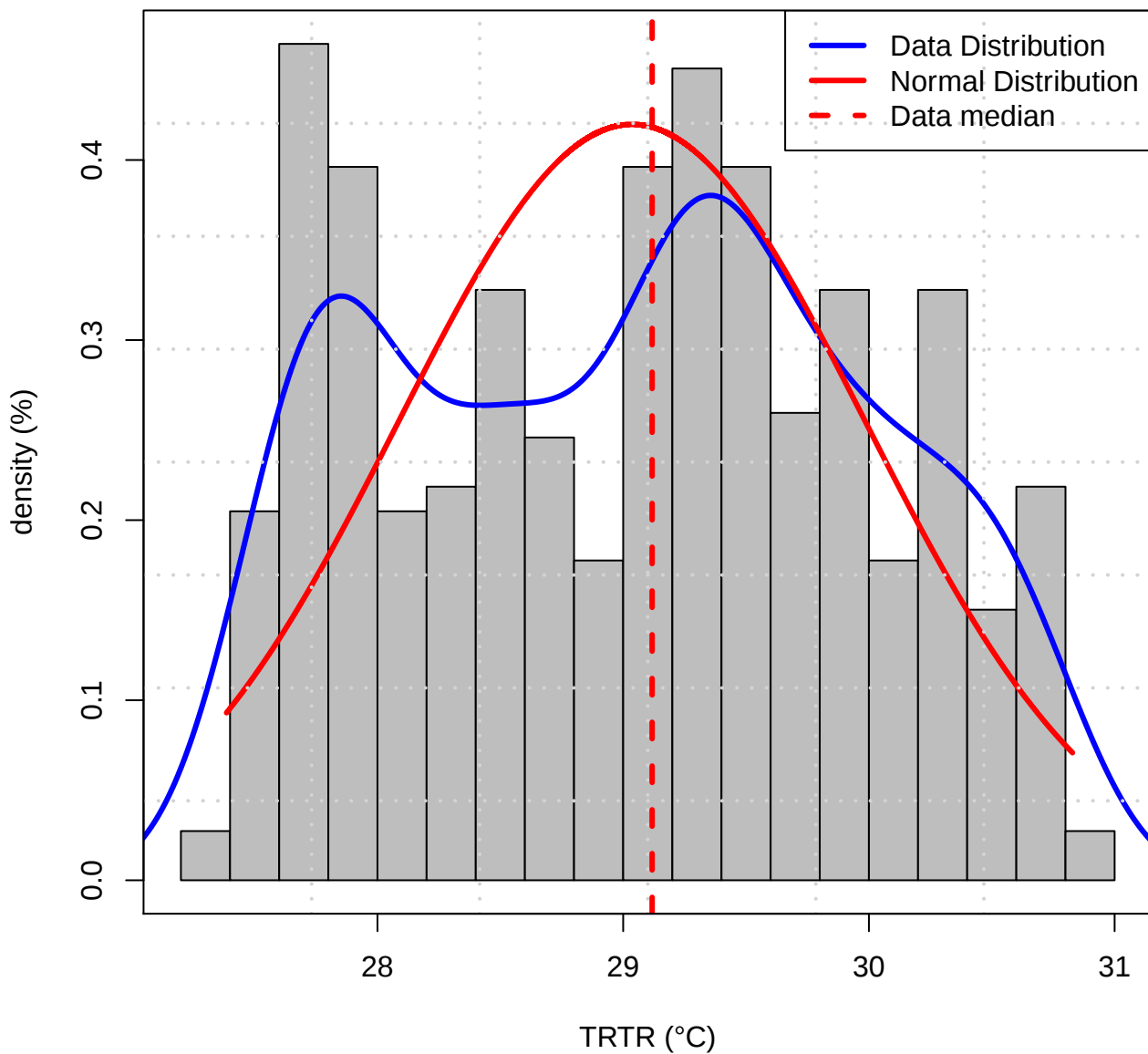
Histogram of Data distribution (TASMAX of TRTR)
