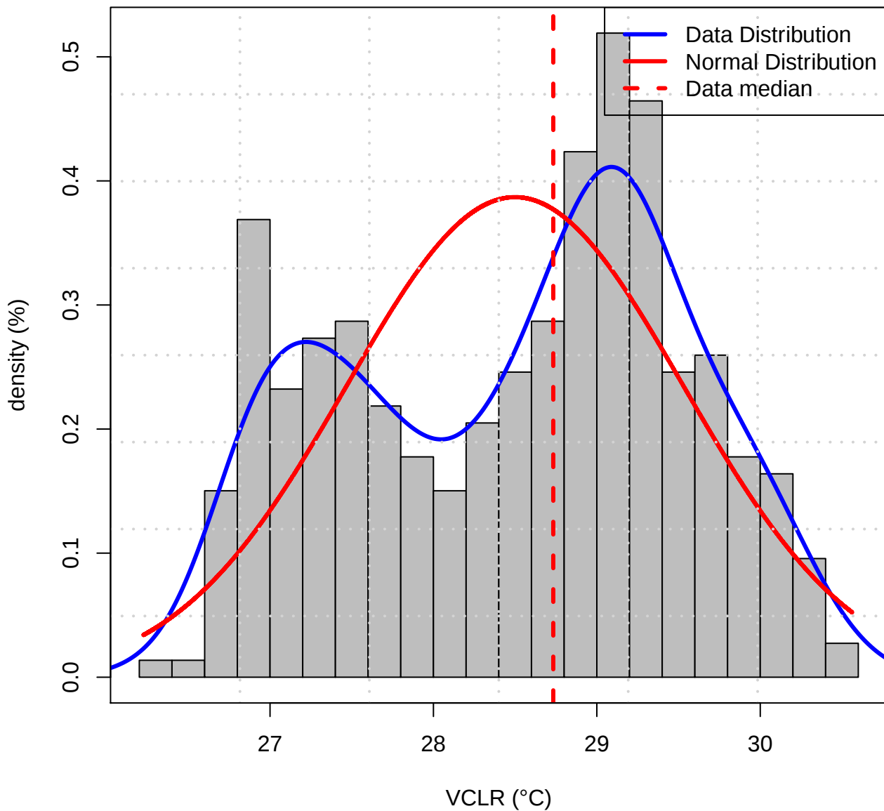
Histogram of Data distribution (TASMAX of VCLR)
