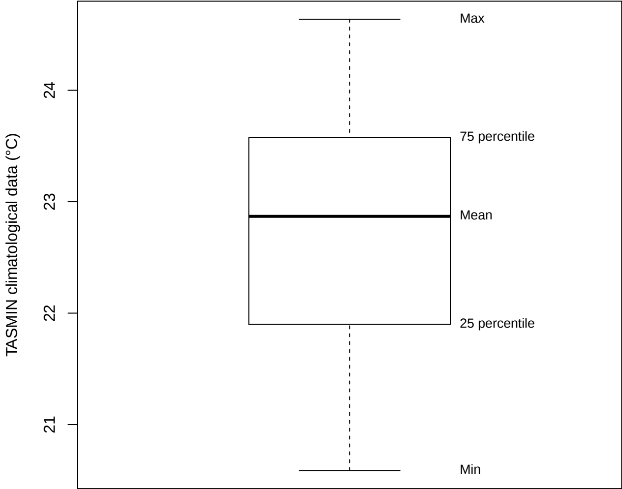
Box plot (TAS of BASP)
