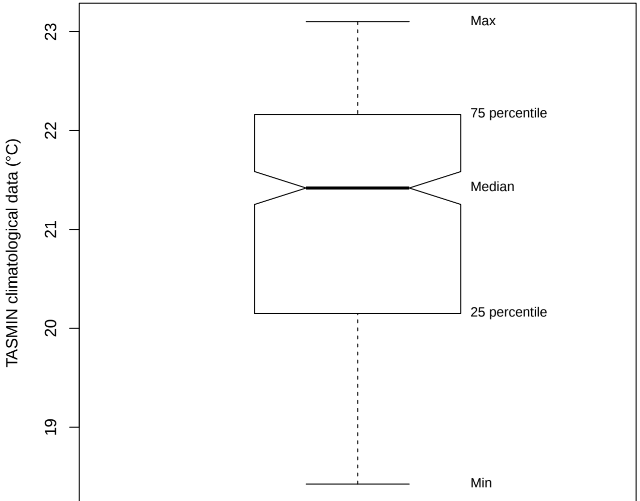
Box plot (TASMIN of AJPB)
