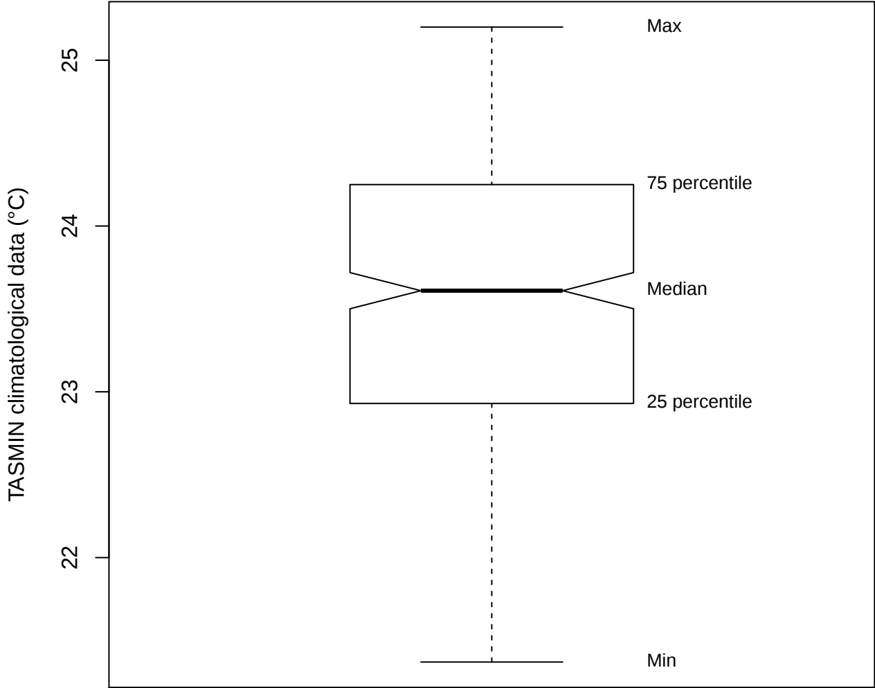
Box plot (TASMIN of DIAM)
