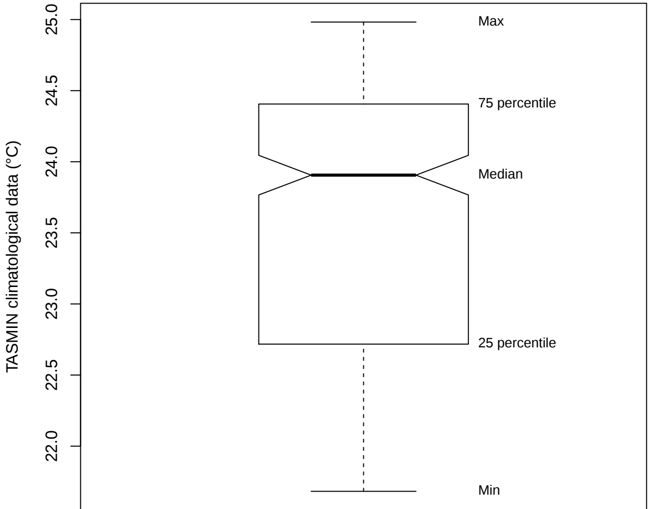
Box plot (TASMIN of FDFD)
