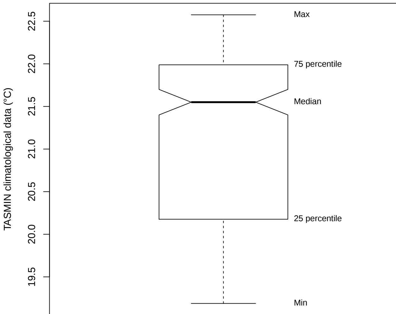
Box plot (TASMIN of FSDC)
