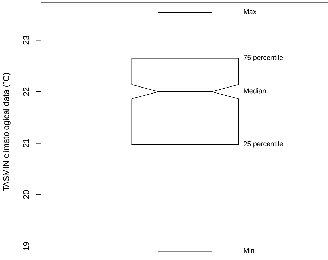
Box plot (TASMIN of FSDG)
