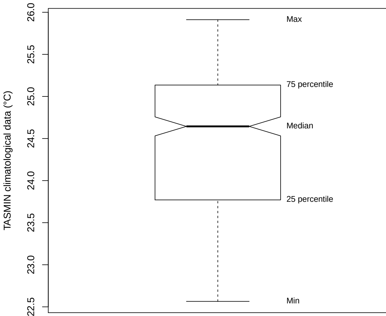
Box plot (TASMIN of LFRC)
