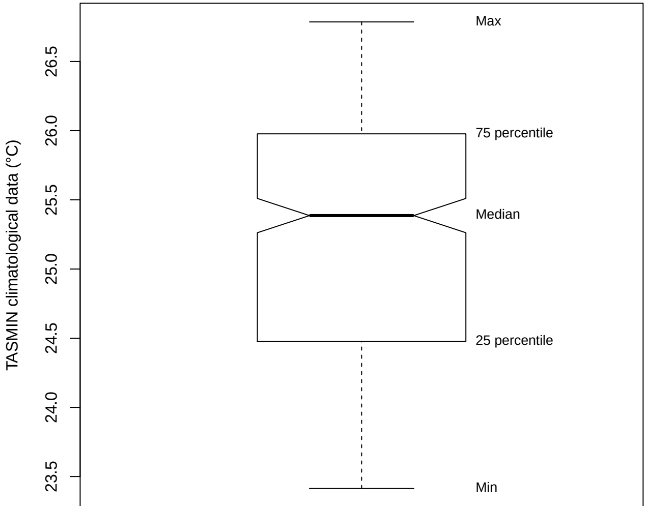
Box plot (TASMIN of ROBP)
