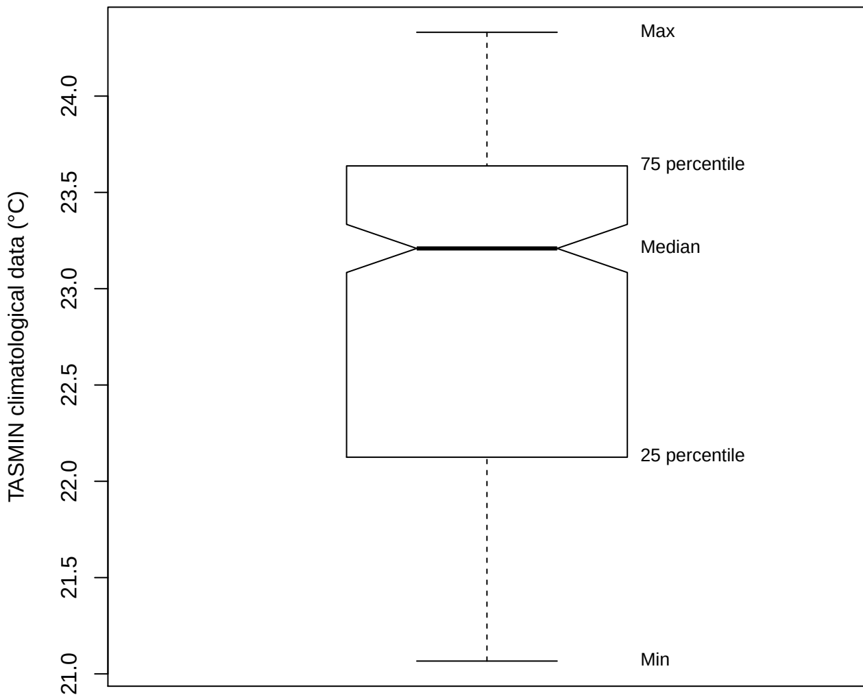
Box plot (TASMIN of STEB)
