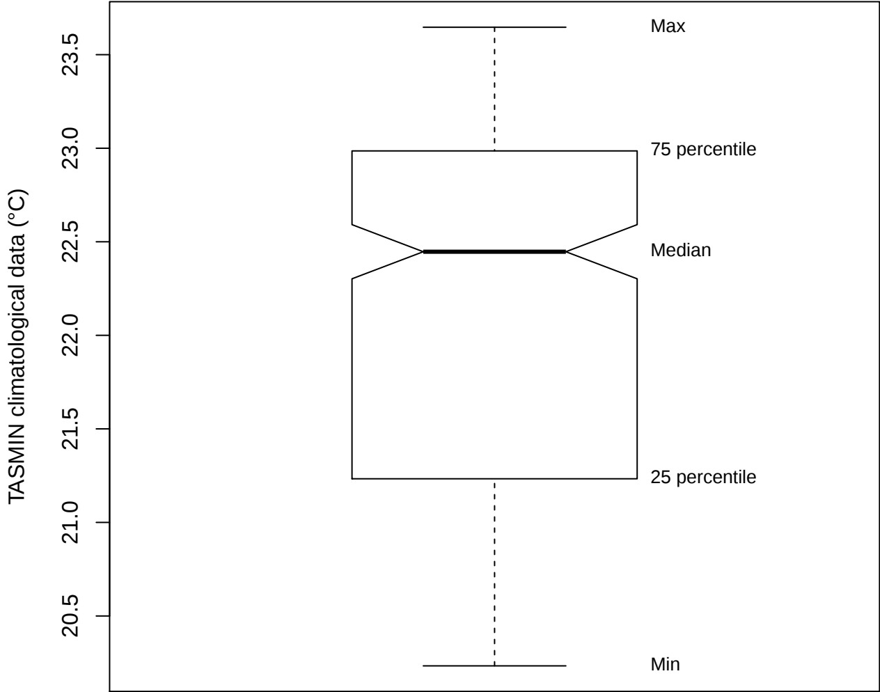
Box plot (TASMIN of STJB)
