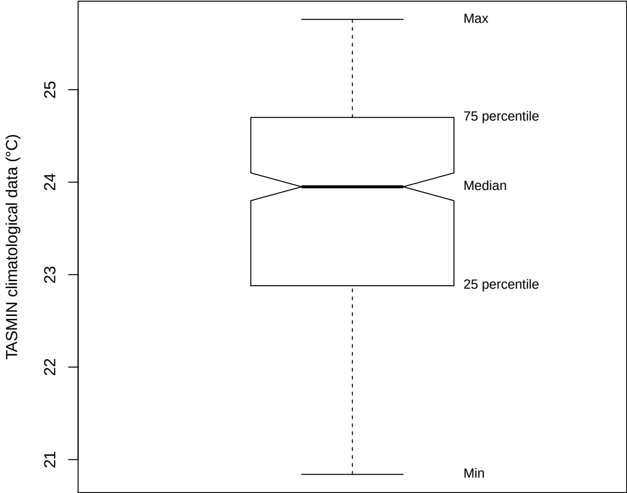
Box plot (TASMIN of STLC)
