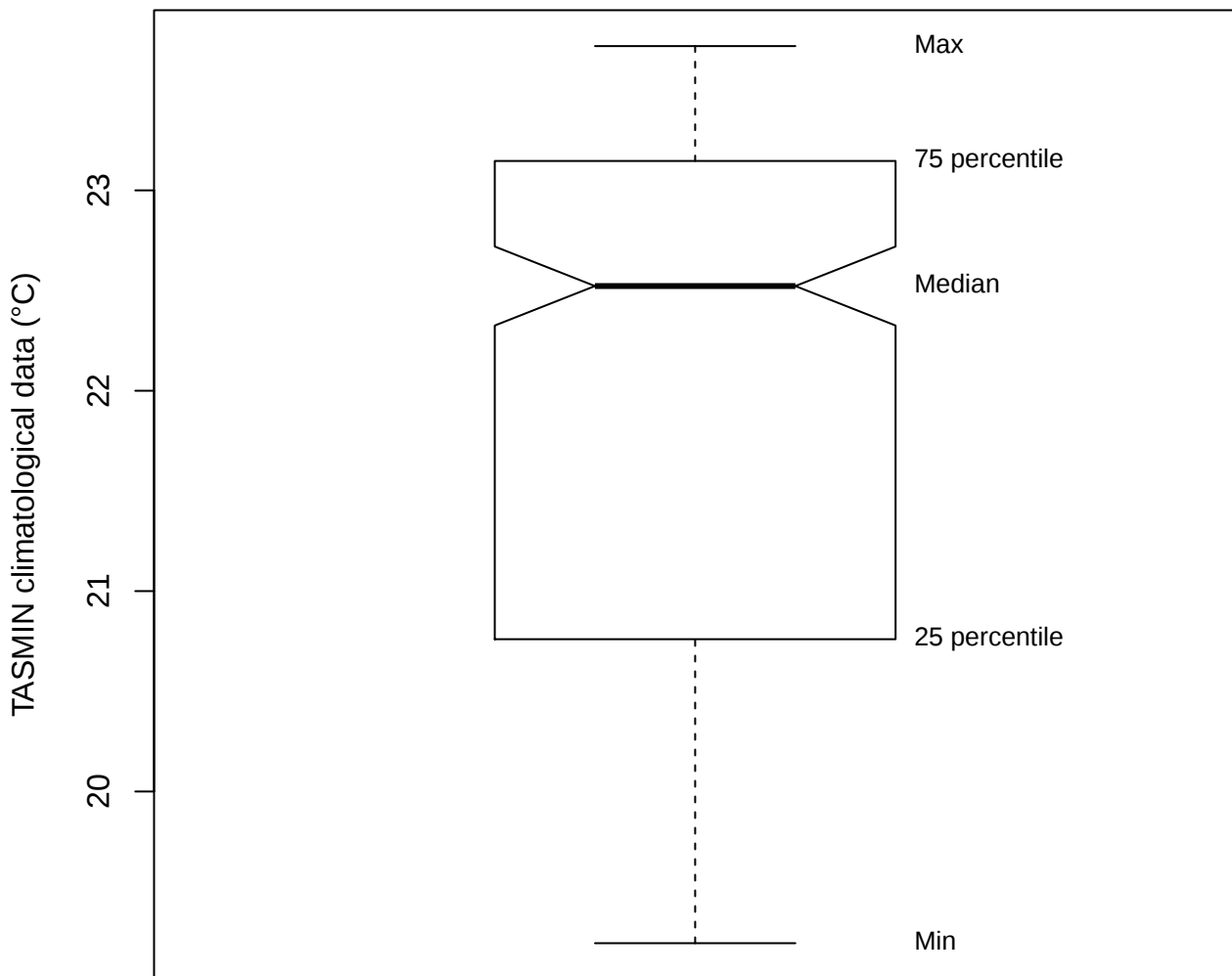
Box plot (TASMIN of TILP)
