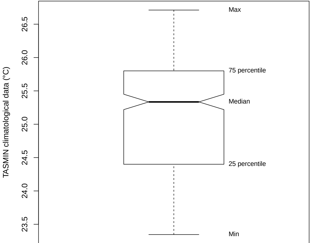
Box plot (TASMIN of TRTC)
