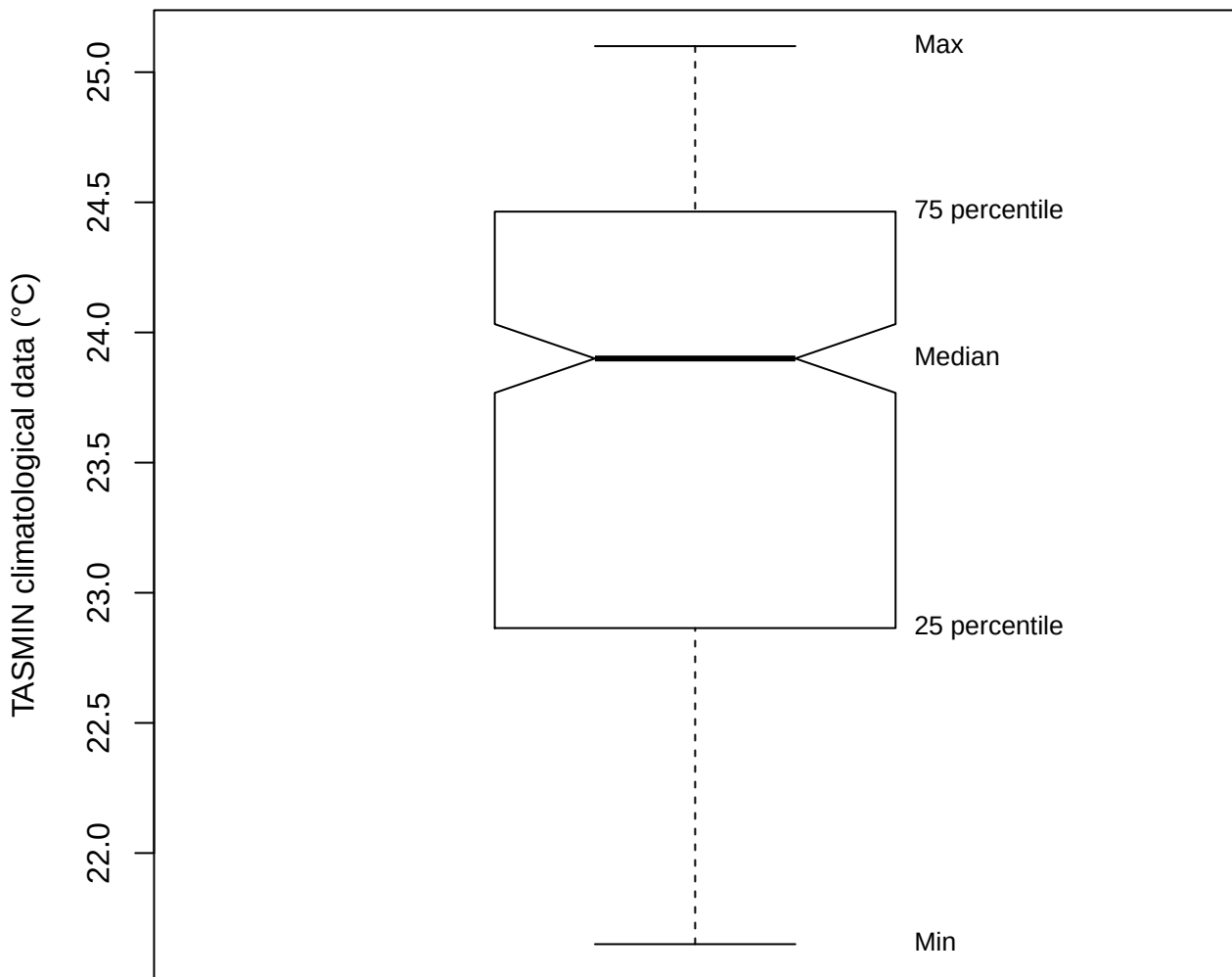
Box plot (TASMIN of TRTR)
