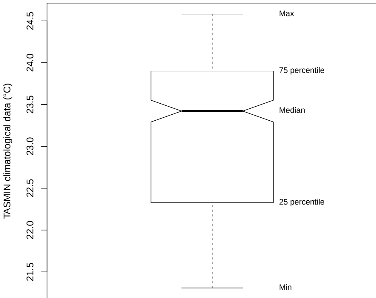
Box plot (TASMIN of VCLR)
