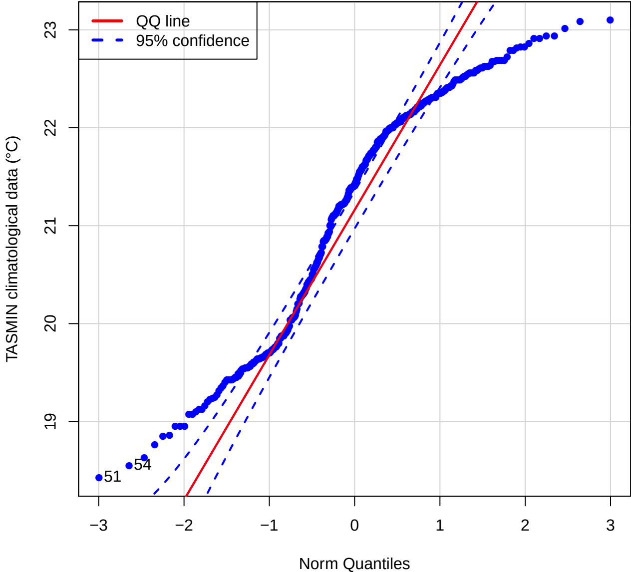
QQ plot (TASMIN of AJPB)
