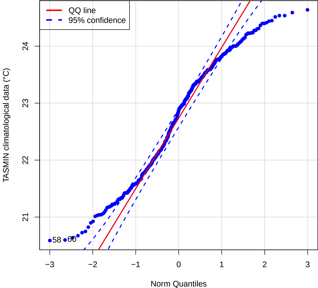
QQ plot (TASMIN of BASP)
