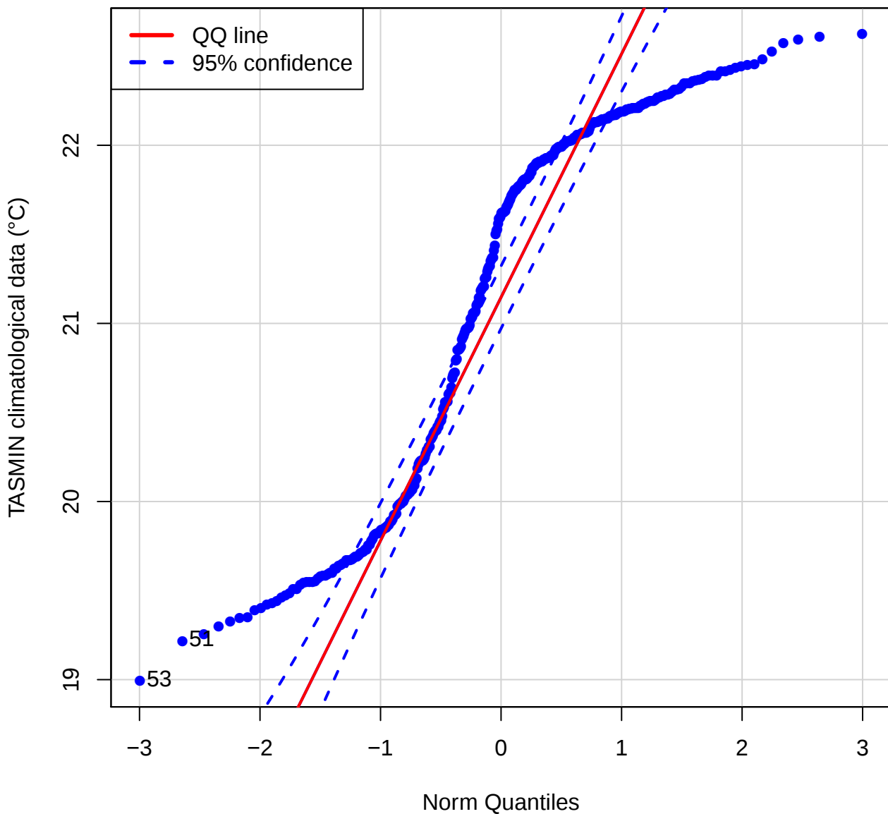
QQ plot (TASMIN of BLLF)
