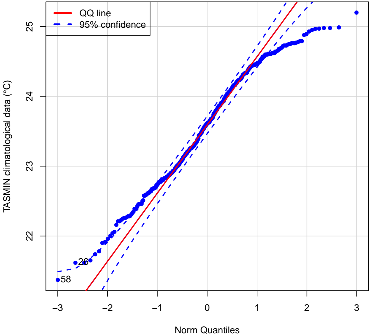
QQ plot (TASMIN of DIAM)
