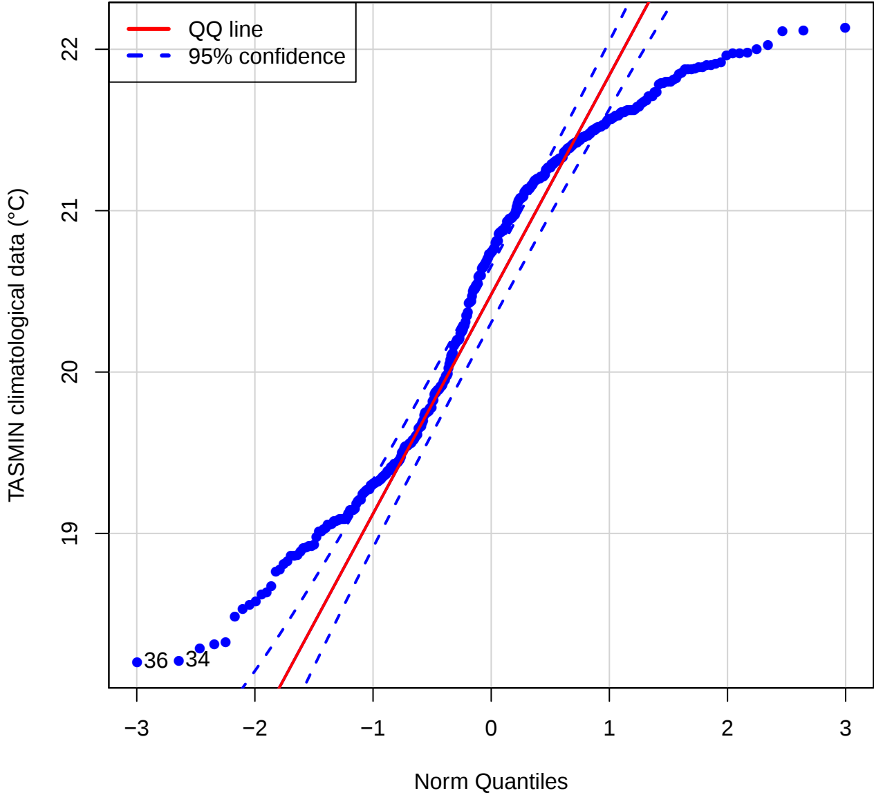
QQ plot (TASMIN of FDFC)
