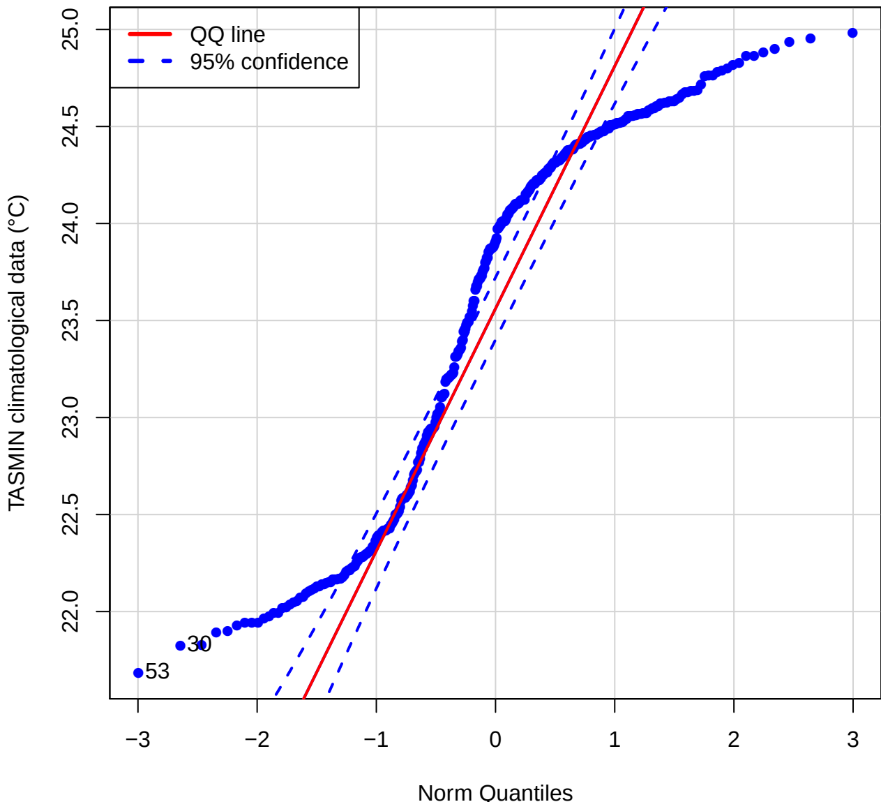
QQ plot (TASMIN of FDFD)
