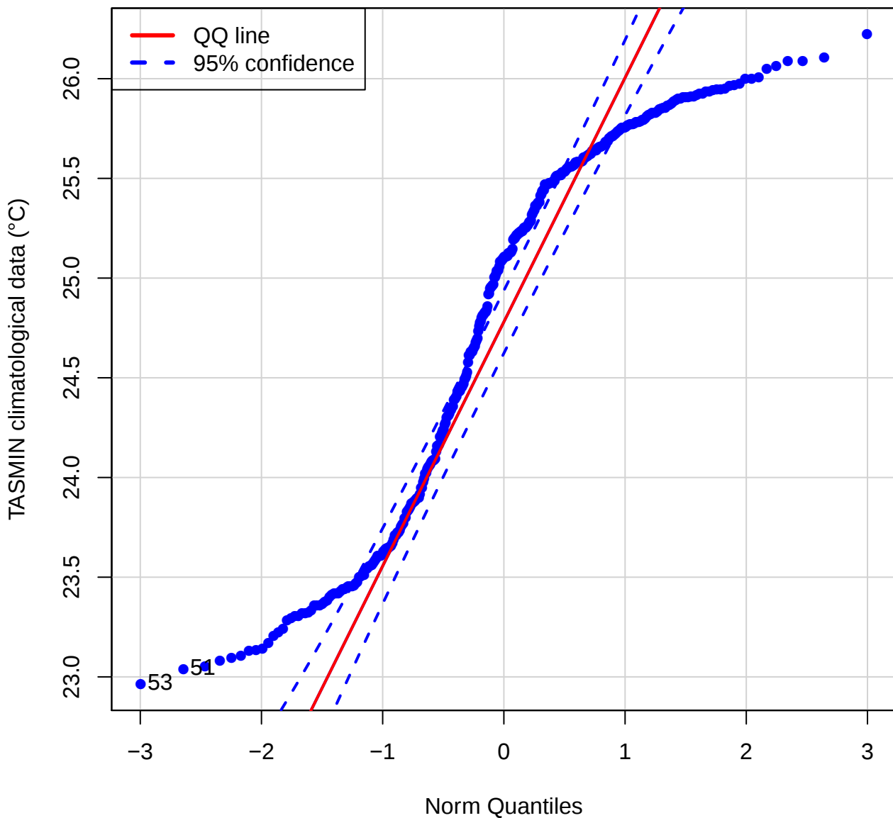
QQ plot (TASMIN of FDFP)
