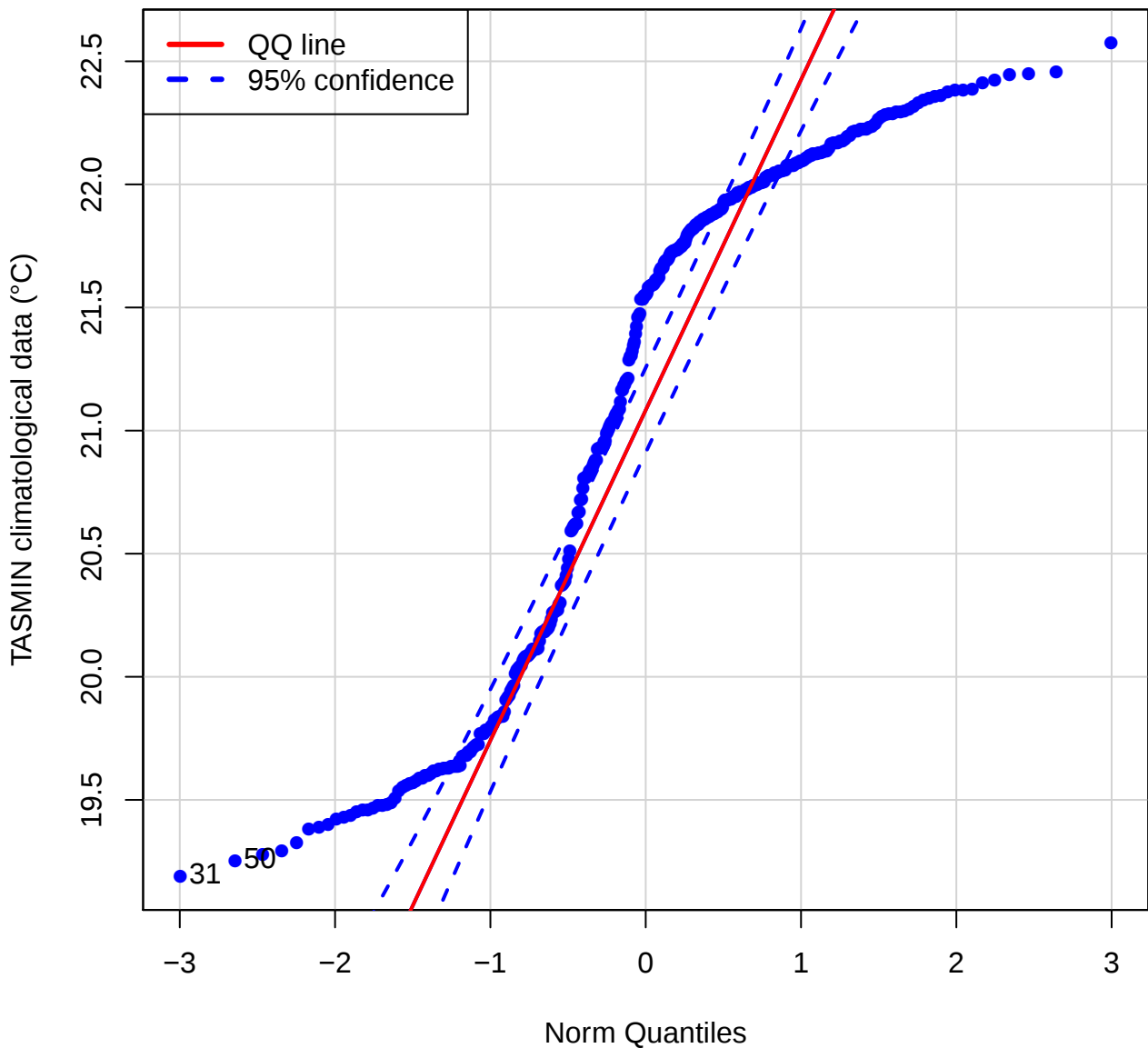
QQ plot (TASMIN of FSDC)
