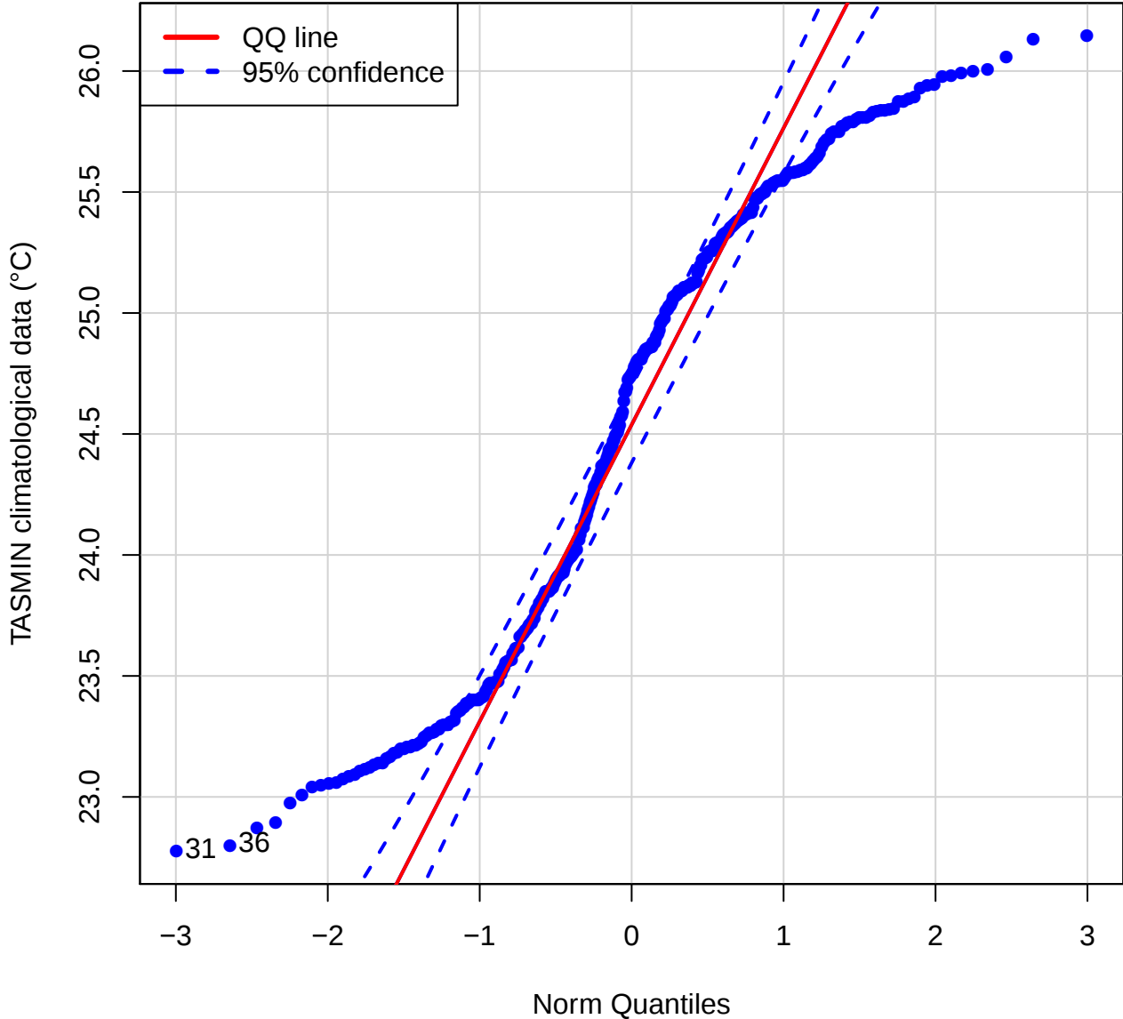
QQ plot (TASMIN of GDRV)
