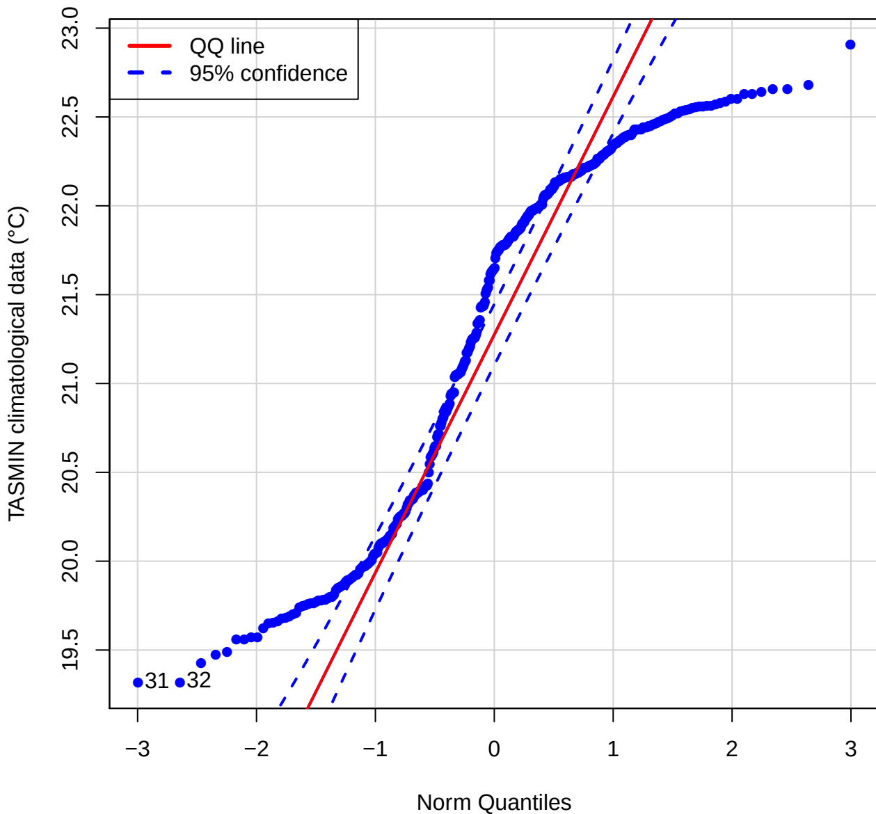
QQ plot (TASMIN of GMRN)
