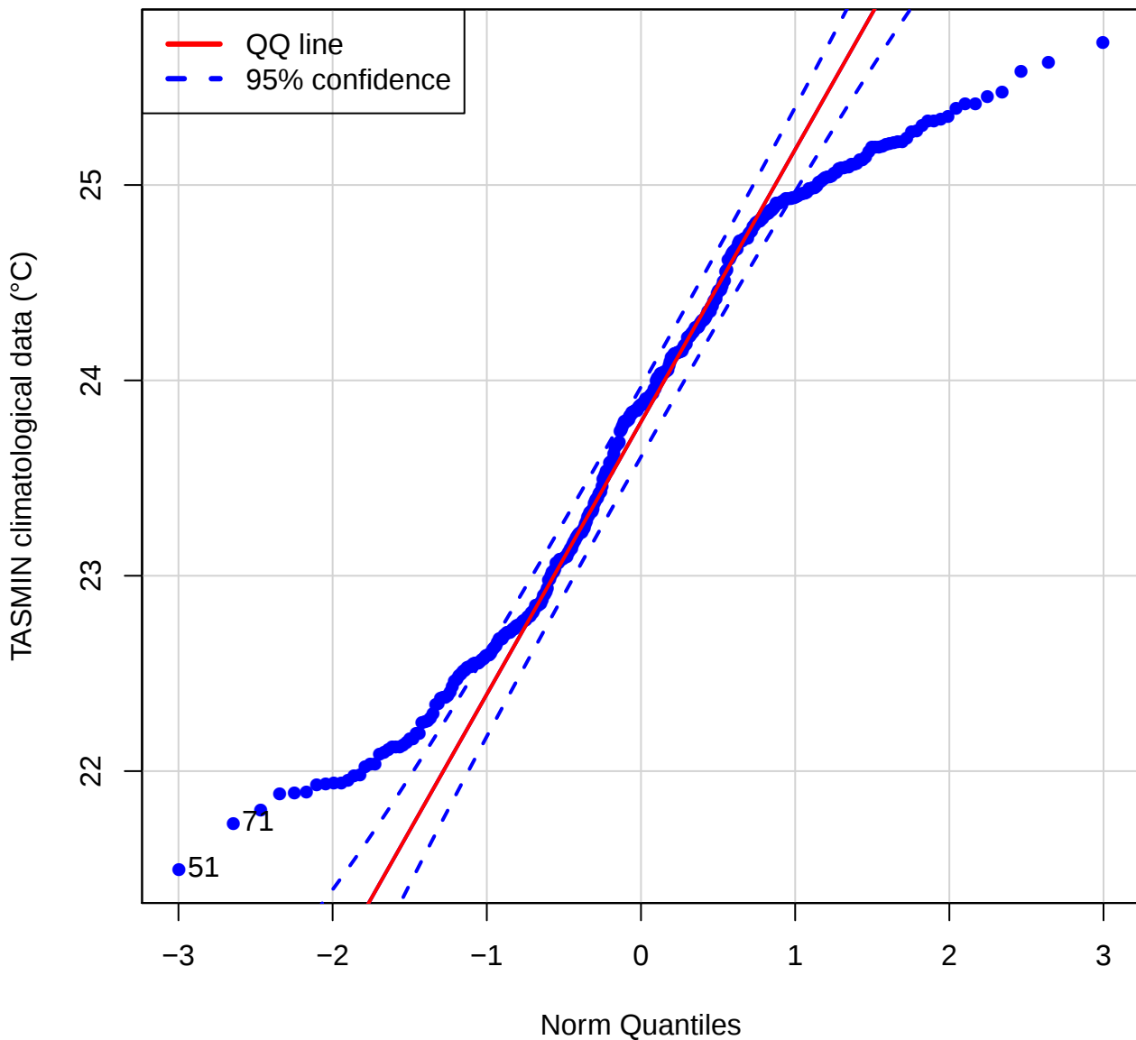
QQ plot (TASMIN of LAMA)
