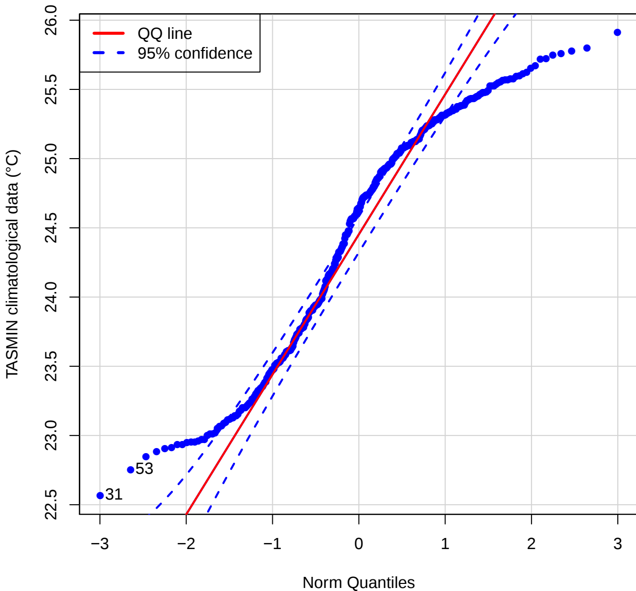
QQ plot (TASMIN of LFRC)
