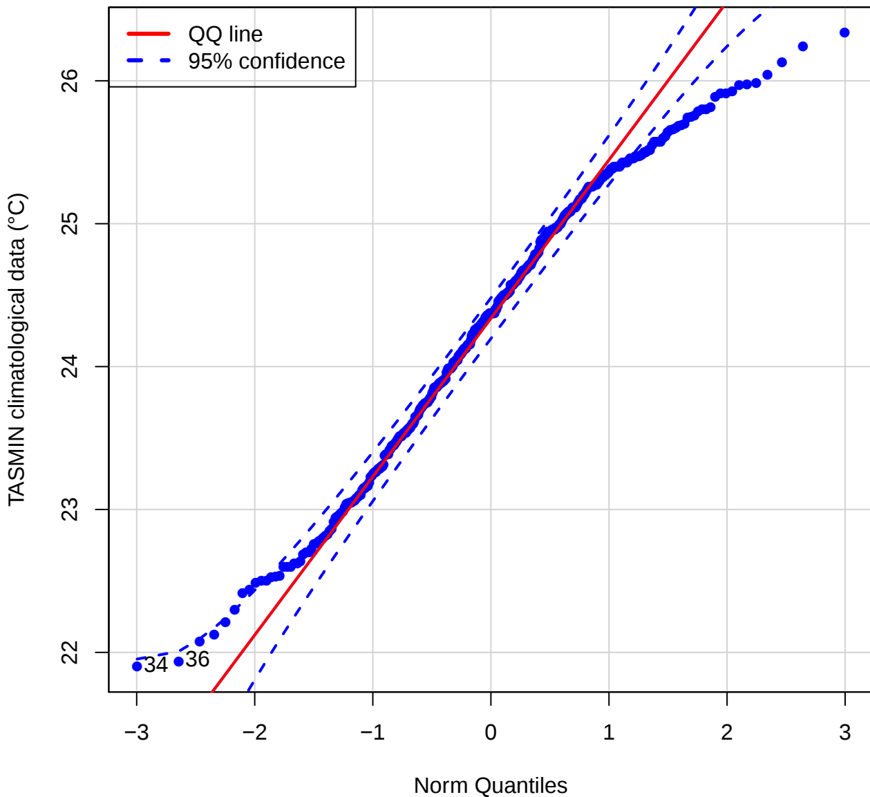
QQ plot (TASMIN of LFRS)
