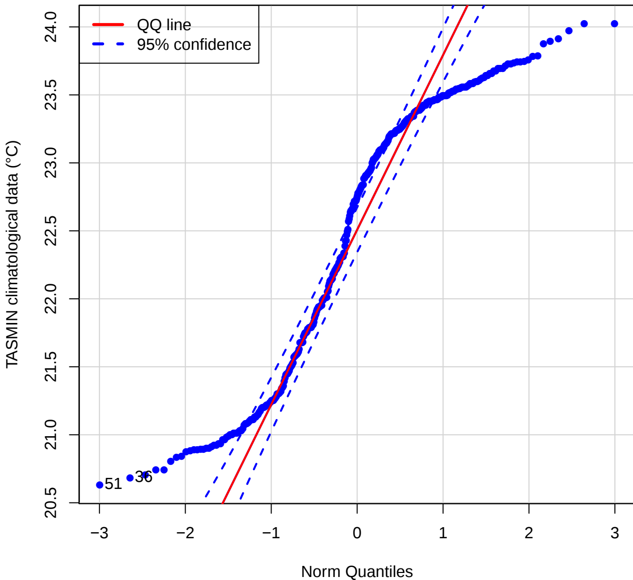
QQ plot (TASMIN of MACB)
