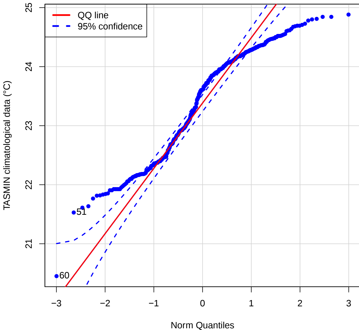
QQ plot (TASMIN of MARB)
