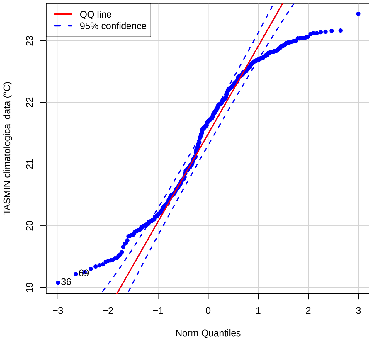
QQ plot (TASMIN of MRRC)
