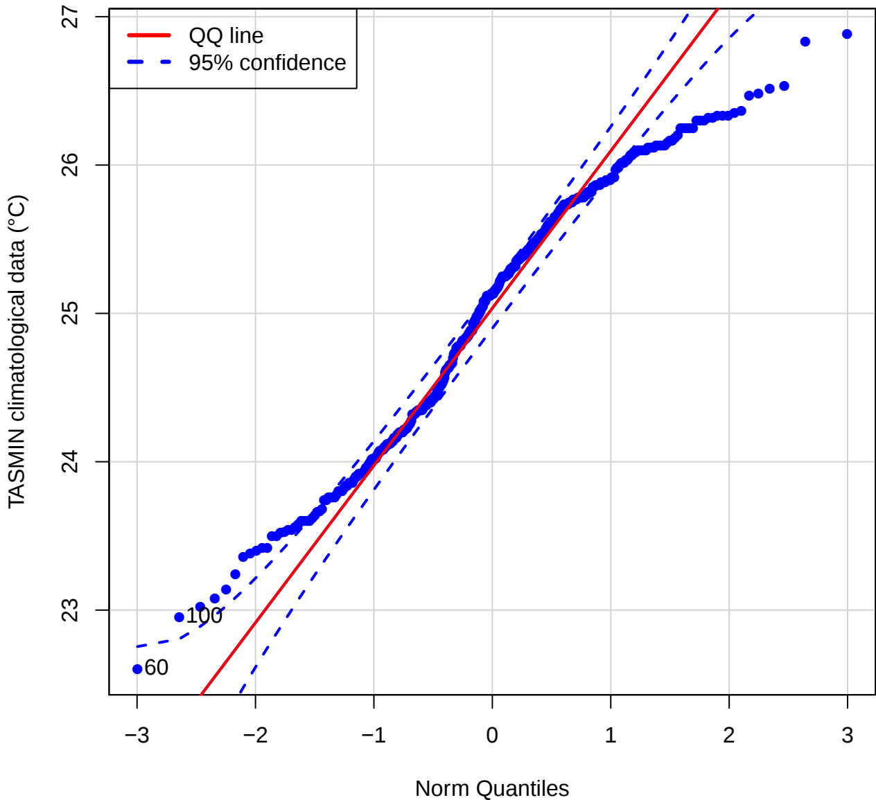
QQ plot (TASMIN of PANS)
