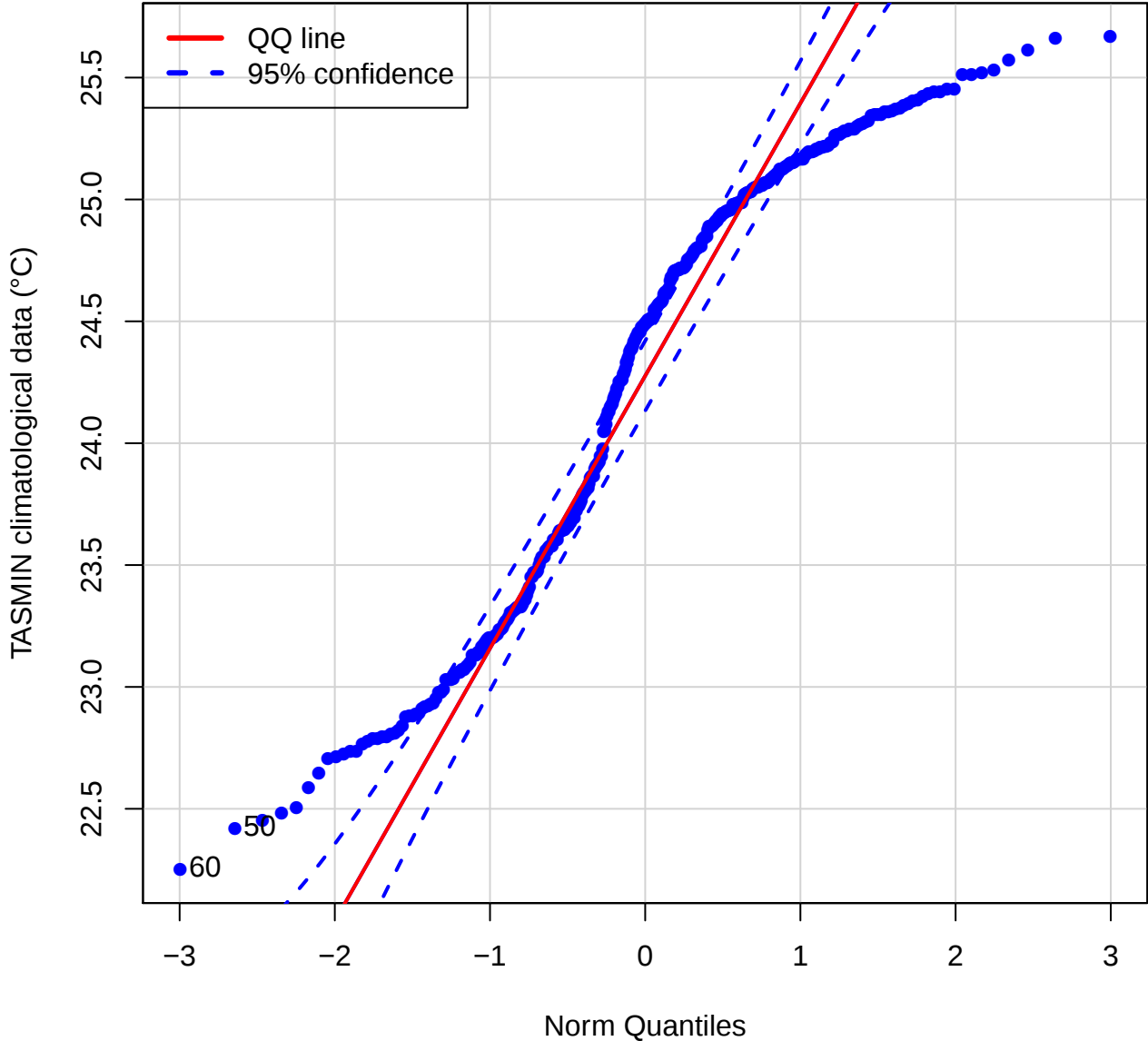
QQ plot (TASMIN of RVPE)
