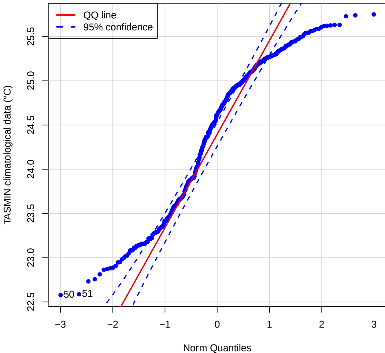
QQ plot (TASMIN of STAN)
