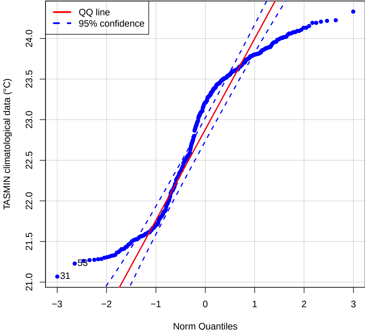
QQ plot (TASMIN of STEB)
