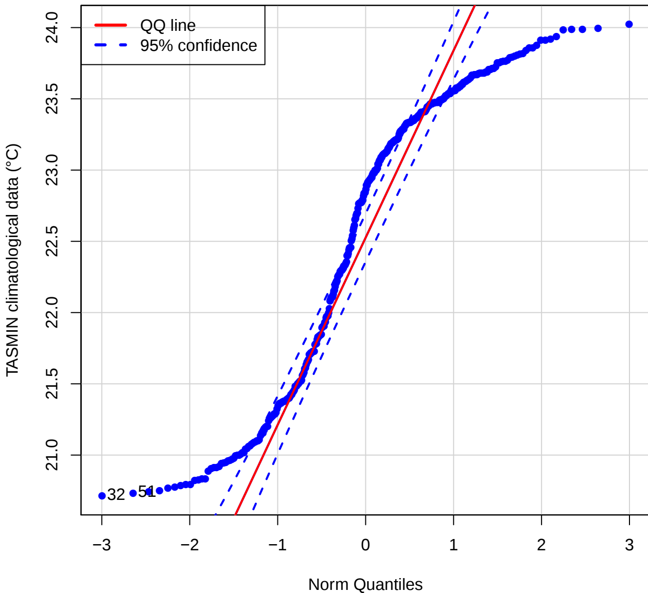
QQ plot (TASMIN of STJO)
